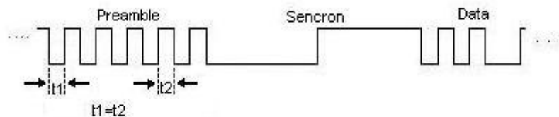
Figure 2. Data Format
